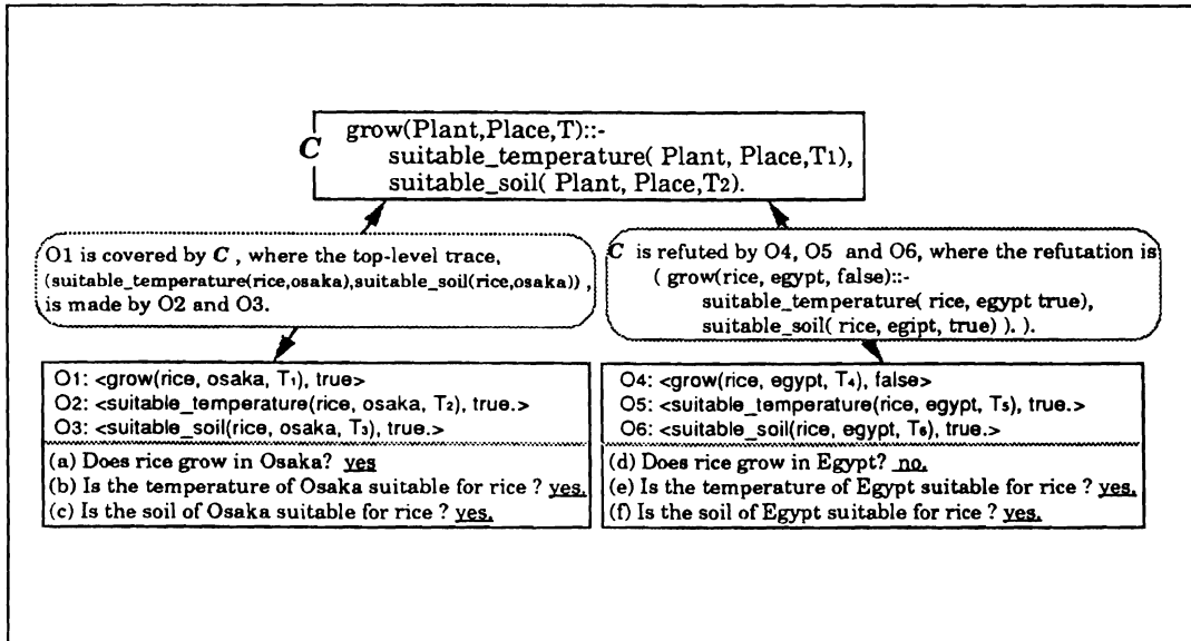
Figure 6. Examples of the top-level trace and the refutation for a clause
